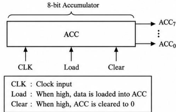
Figure 3.4 Accumulator Register
