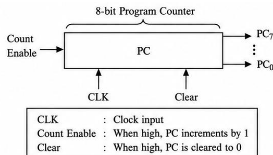
Figure 3.5: Program Counter
