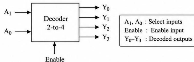
Figure 3.7: Decoder
